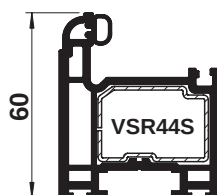
Standard Sash
